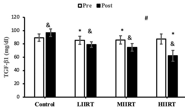
FIGURE 6 | Pre and post-training values (mean \pm SD) for TGF-β1 in control, low-intensity interval resistance training (LIIRT), moderate-intensity interval resistance training (MIIRT), high-intensity interval resistance training (HIIRT) groups. *Significant differences from the control group ( p < 0.05 ). &Significant differences from pretest values ( p < 0.05 ). #Significant differences between training groups ( p < 0.05 ).
