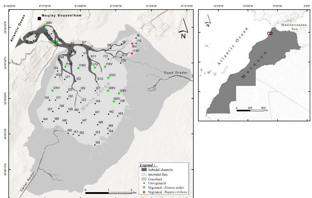
Figure 1. Map showing the location of the Moulay Bouselham lagoon and sampling stations. S: subtidal; I: intertidal; V: vegetated.
