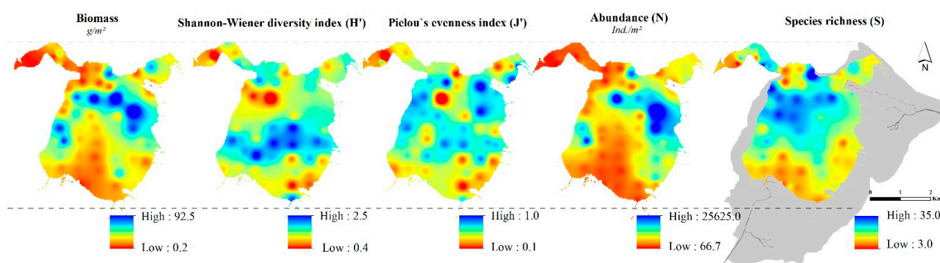
Figure 3. Interpolation of the spatial distribution of species richness (S), abundance (N), diversity index (H'), equitability index (J') and the biomass in the Moulay Bousselham lagoon.
