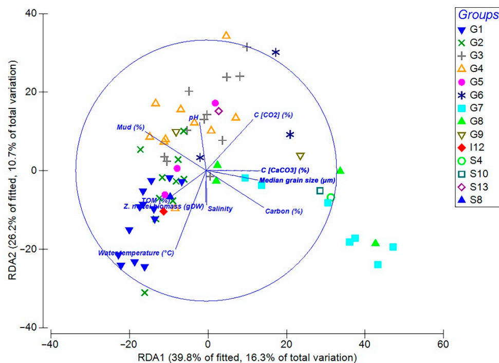
Figure 7. Two-dimensional redundancy analysis (RDA) ordination representing the model of spatial variation in macrozoobenthos community structure related to the predictor variables selected through the best linear models based on distance (DISTLM).
