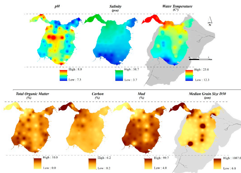
Figure 2. Maps showing the spatial distribution of environmental variables in the Moulay Bousseham lagoon.
